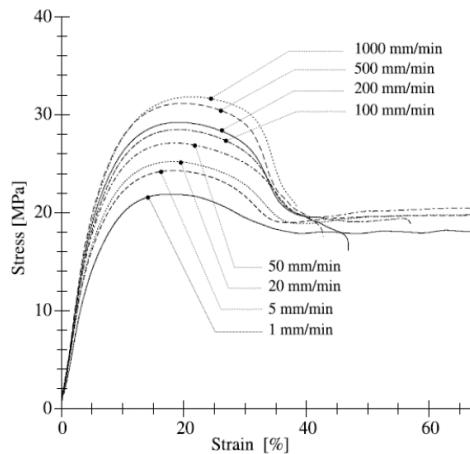
Fig 1. Variation of stress-strain response with respect to crosshead speed for natural PP-R material (Shahin and Yayla, 2005)
